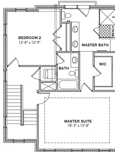
Third Floor
